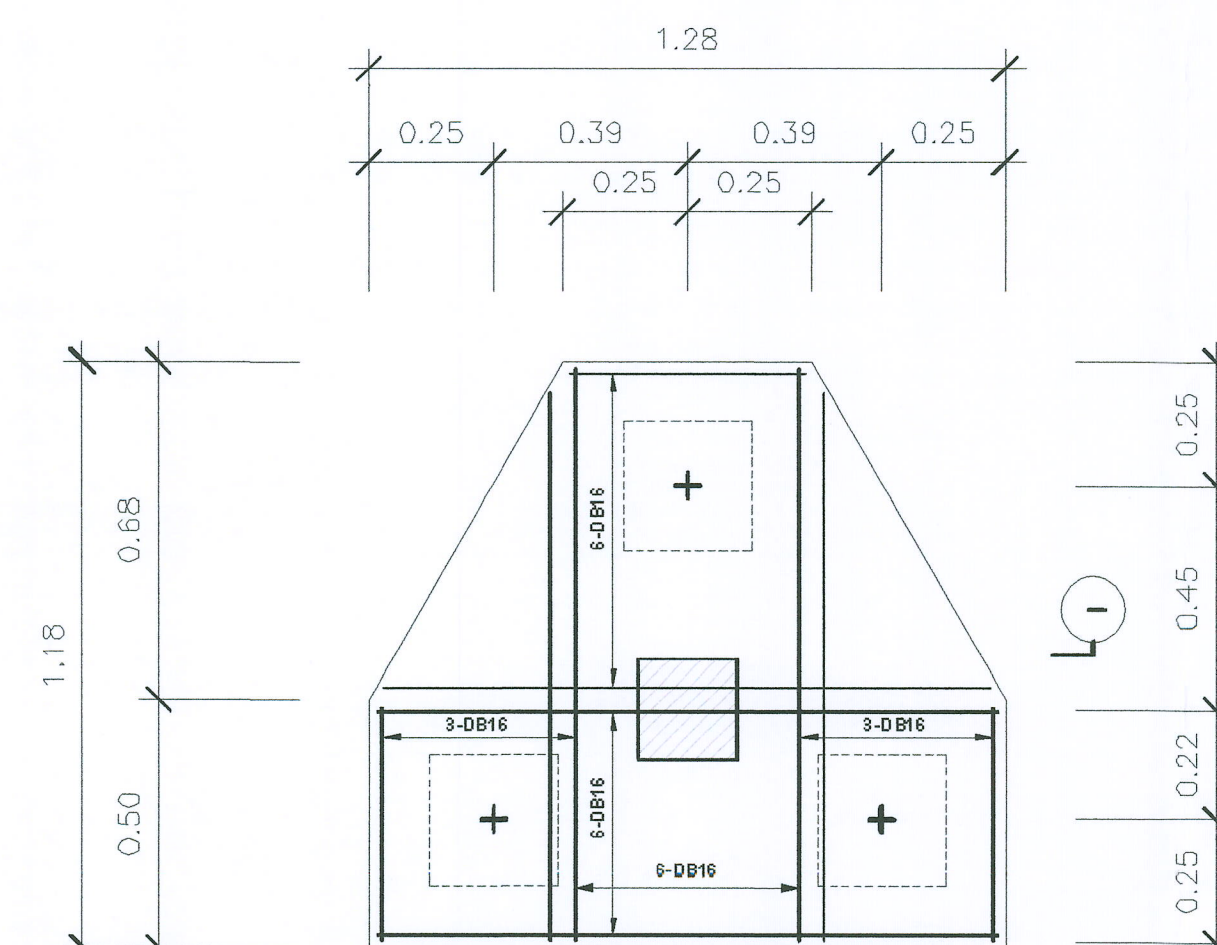
PLAN F326 SCALE 1:25
