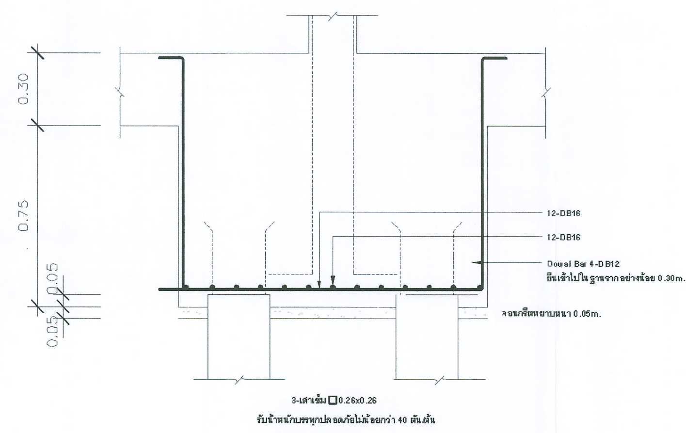
SECTION F326 SCALE 1:25
