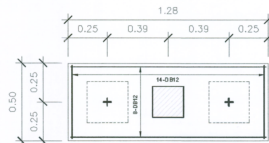
PLAN F226 SCALE 1:25
