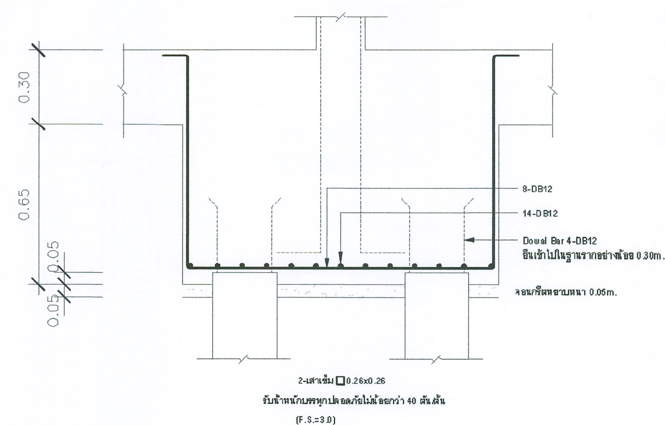
SECTION F226 SCALE 1:25
