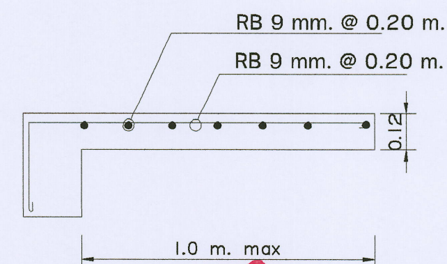
SLAB CROSS SECTION SC
