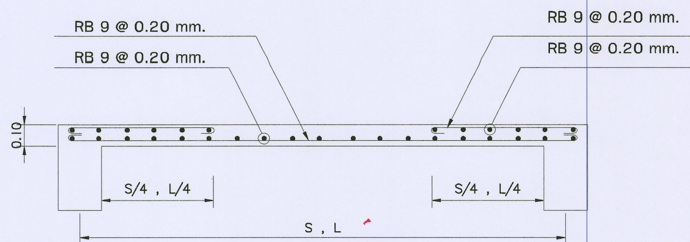
SLAB CROSS SECTION S2
