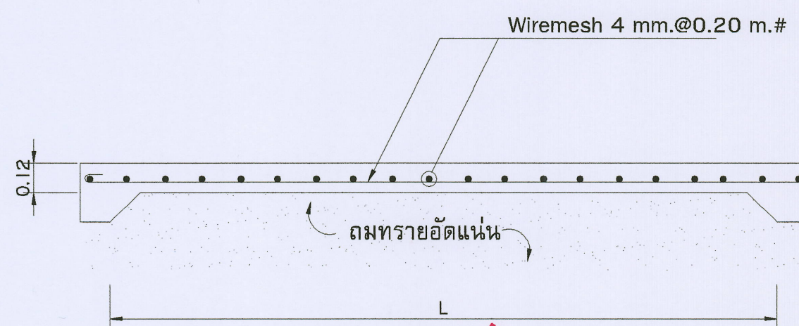
GROUND SLAB CROSS SECTION GS
