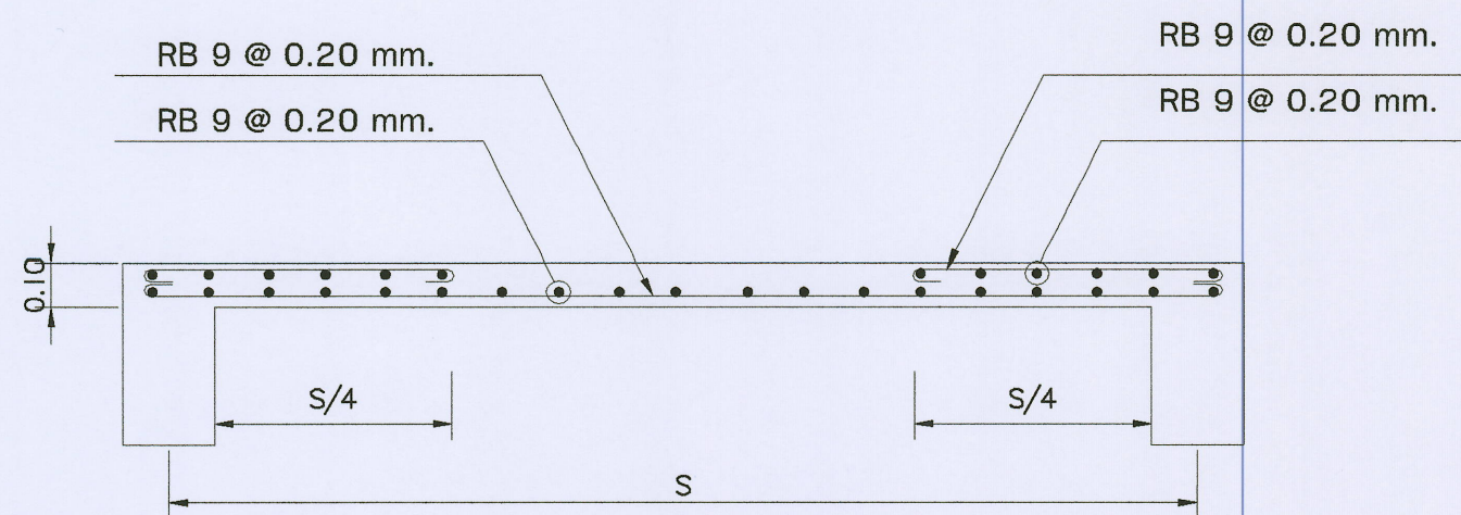
SLAB CROSS SECTION S1
