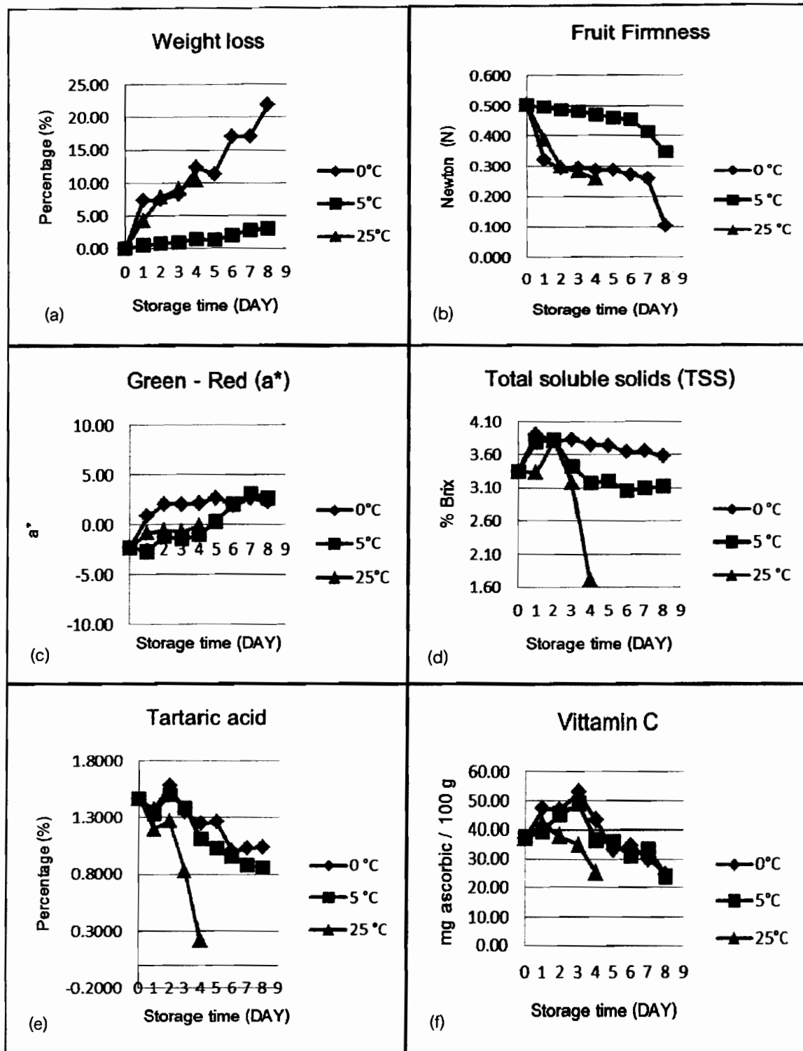
Figure 1 Change of physical and chemical properties of bilimbi at storage time.
